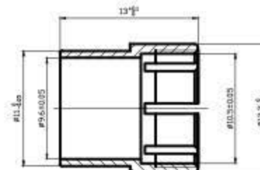
Clamp
